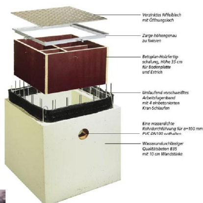
Pumpensumpf
